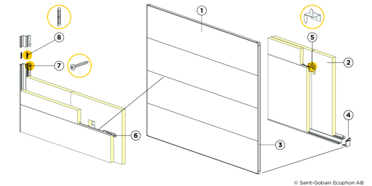
Installation diagram (M720) for Ecophon Akusto Wall Bass horizontal installation with Connect shadow profiles.
