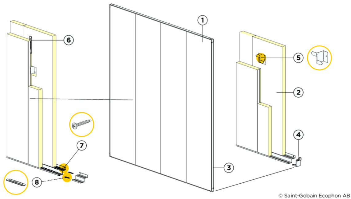
Installation diagram (M719) for Ecophon Akusto Wall C Extra Bass vertical installation with Connect shadow profiles.
