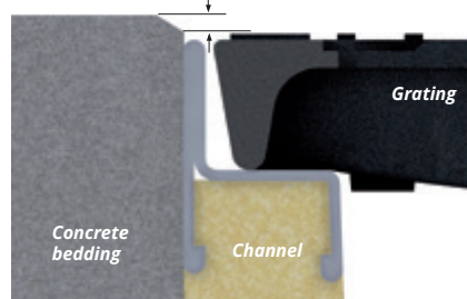
Detail A Channel with edge 3-5mm from the edge
