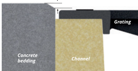
Detail B Channel without edge 3-5mm from the grating
