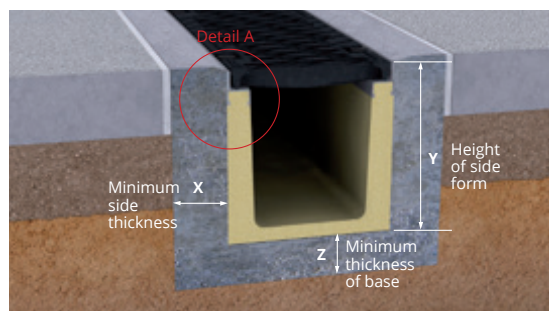
Detail A Channel with edge 3-5mm from the edge
